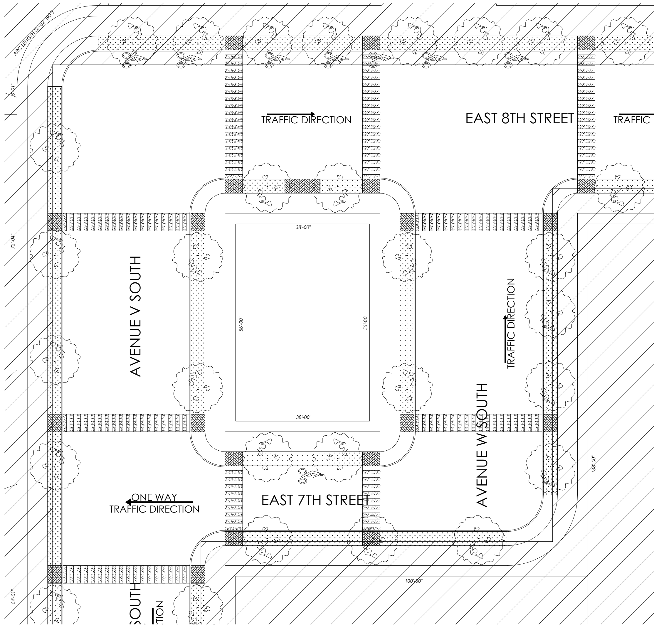
1 BLOCK 01 048 - BLOCK PLAN
